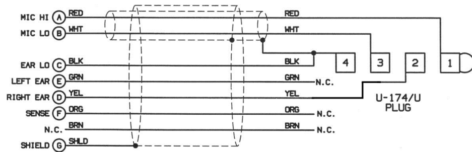
Figure 1: Cable Schematic (41035G-03)
